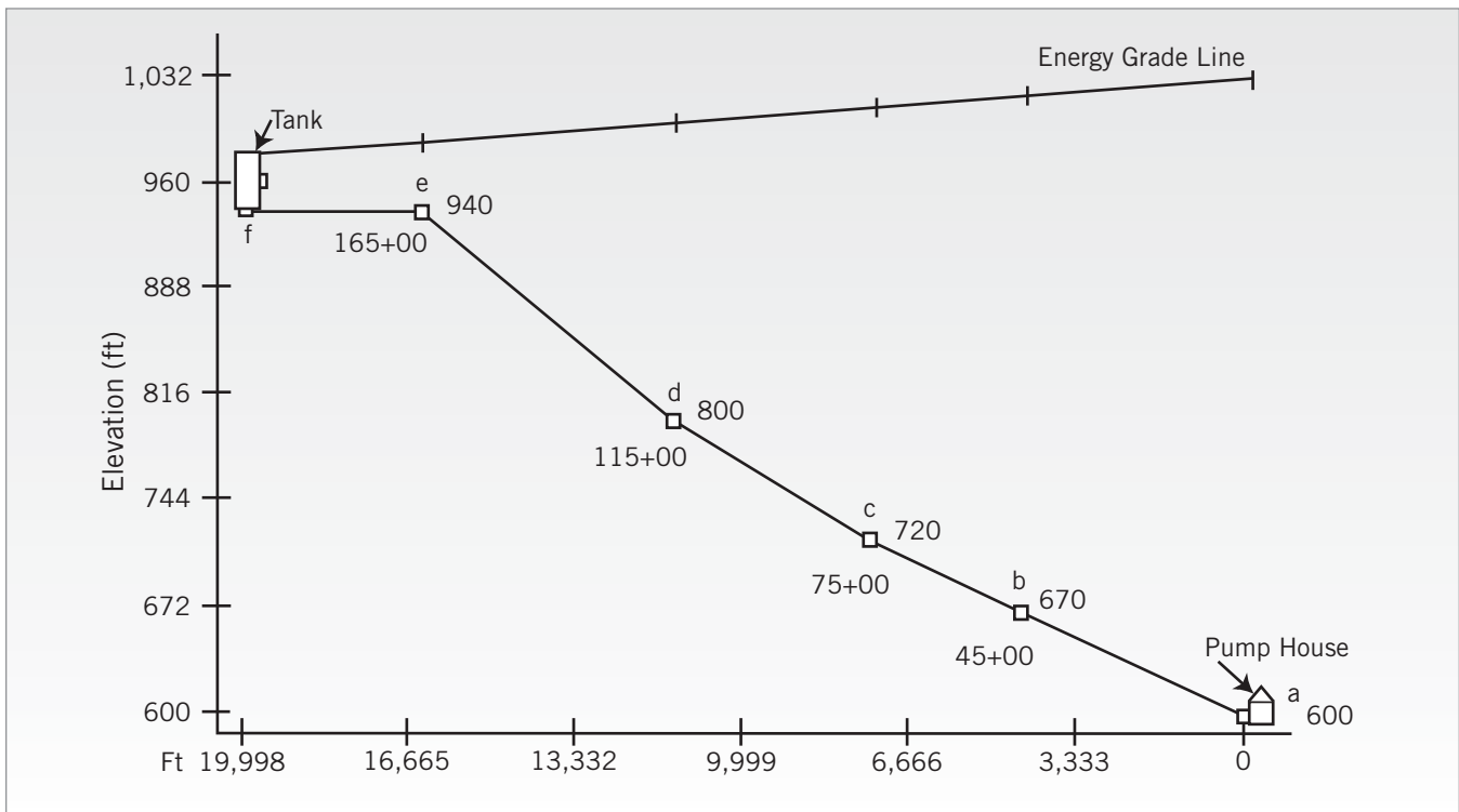
Figure 4 – Pipeline Profile
